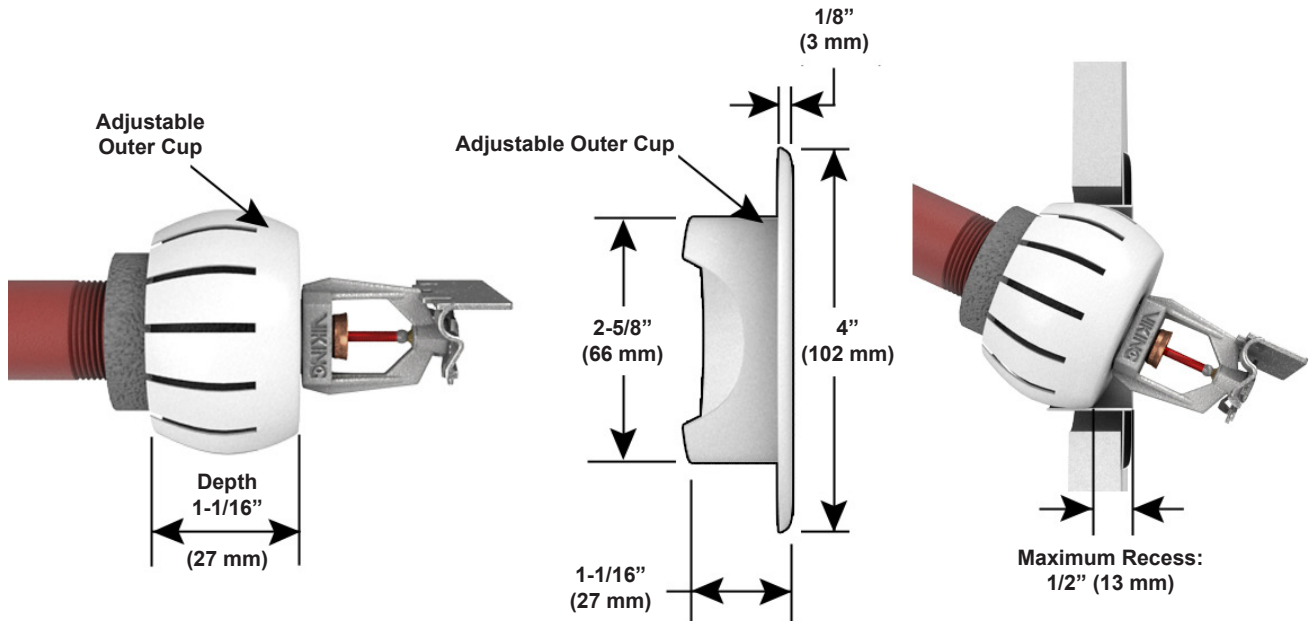
Figure 4: Installation of the Model G-1 Recessed Escutcheon with up to 1/2" (12.7 mm) Adjustment.
