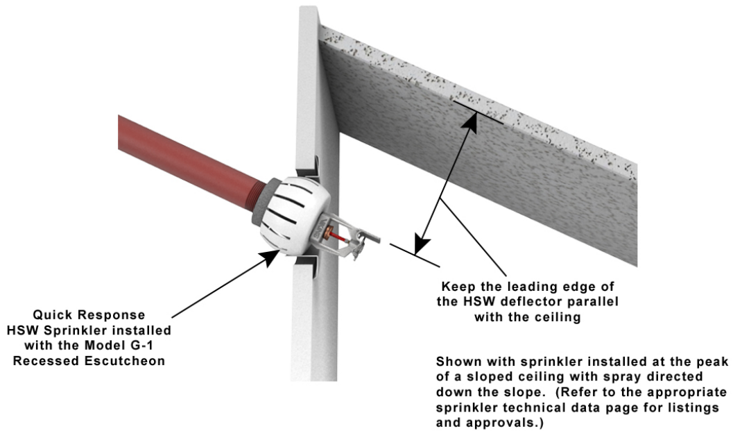
Figure 5: Model G-1 Recessed Escutcheon Installed with a Residential HSW Sprinkler below a sloped ceiling.
